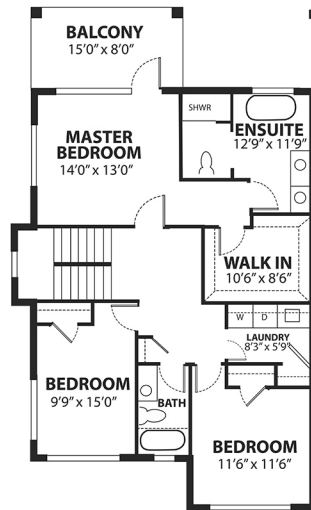
PLAN A - UPPER FLOOR PLAN 1042 SQ FT
